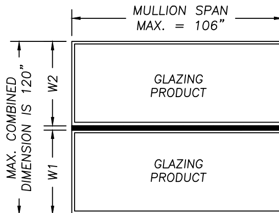
SINGLE MULLED OVER SINGLE
