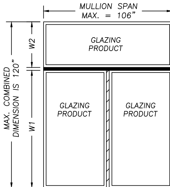
TRANSOM MULLED OVER MULLED SINGLES
