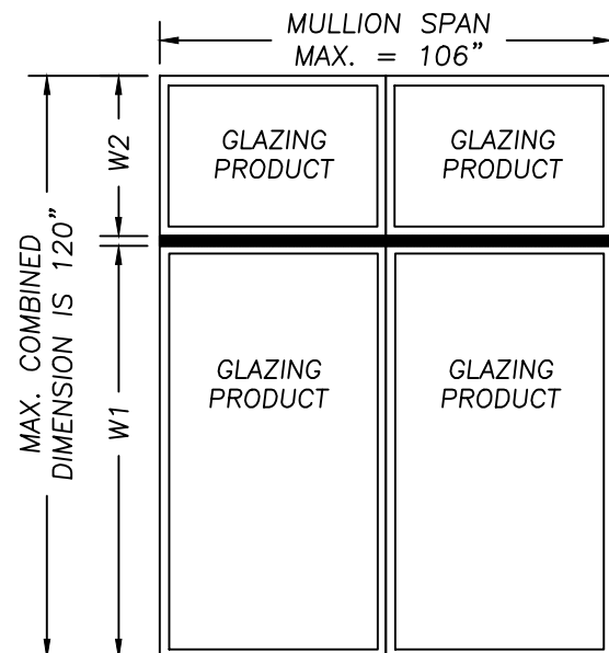
TWIN TRANSOMS MULLED OVER TWINS
