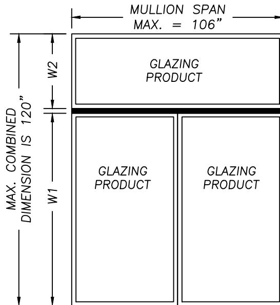
TRANSOM MULLED OVER TWINS
