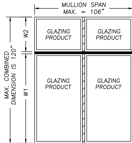
MULLED TRANSOM SINGLES MULLED OVER MULLED SINGLES
